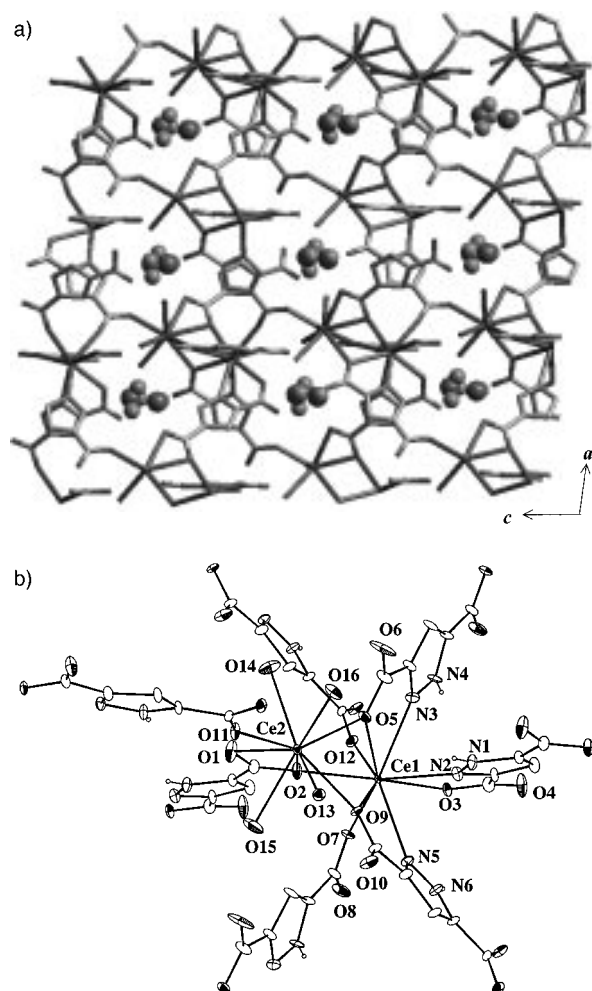
Figure 1. a) View of [\text{Ln}_2(\text{Hpdc})_3(\text{H}_2\text{O})_4] \cdot 2\text{H}_2\text{O} , \text{Ln} = \text{La} ( 2 ), \text{Ln} = \text{Ce} ( 3 ), along the b axis. Large and small solid spheres represent O and H atoms of the uncoordinated water molecules. b) ORTEP drawing of 3 . Both Ce1 and Ce2 atoms are nine coordinate. Selected distances [Å]: Ce1–Ce2 4.0381(12), Ce1–O7 2.427(5), Ce1–O3 2.456(5), Ce1–O12 2.458(5), Ce1–O2 2.469(5), Ce1–O5 2.610(5), Ce1–O9 2.616(4), Ce1–N5 2.628(6), Ce1–N3 2.632(7), Ce1–N2 2.654(6), Ce2–O16 2.413(5), Ce2–O11 2.427(5), Ce2–O13 2.530(5), Ce2–O15 2.541(6), Ce2–O5 2.547(5), Ce2–O1 2.589(5), Ce2–O9 2.595(4), Ce2–O14 2.596(6), Ce2–O2 2.668(5).
